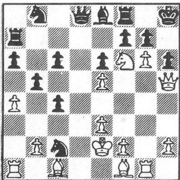
127 After 19...Be8
